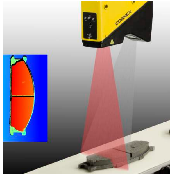
Figure 15. 3D inspection system using a single camera.
