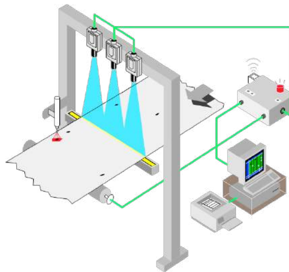
Figure 10. 1D vision systems scan one line at a time while the process moves. In the above example, a defect in the sheet is detected.
