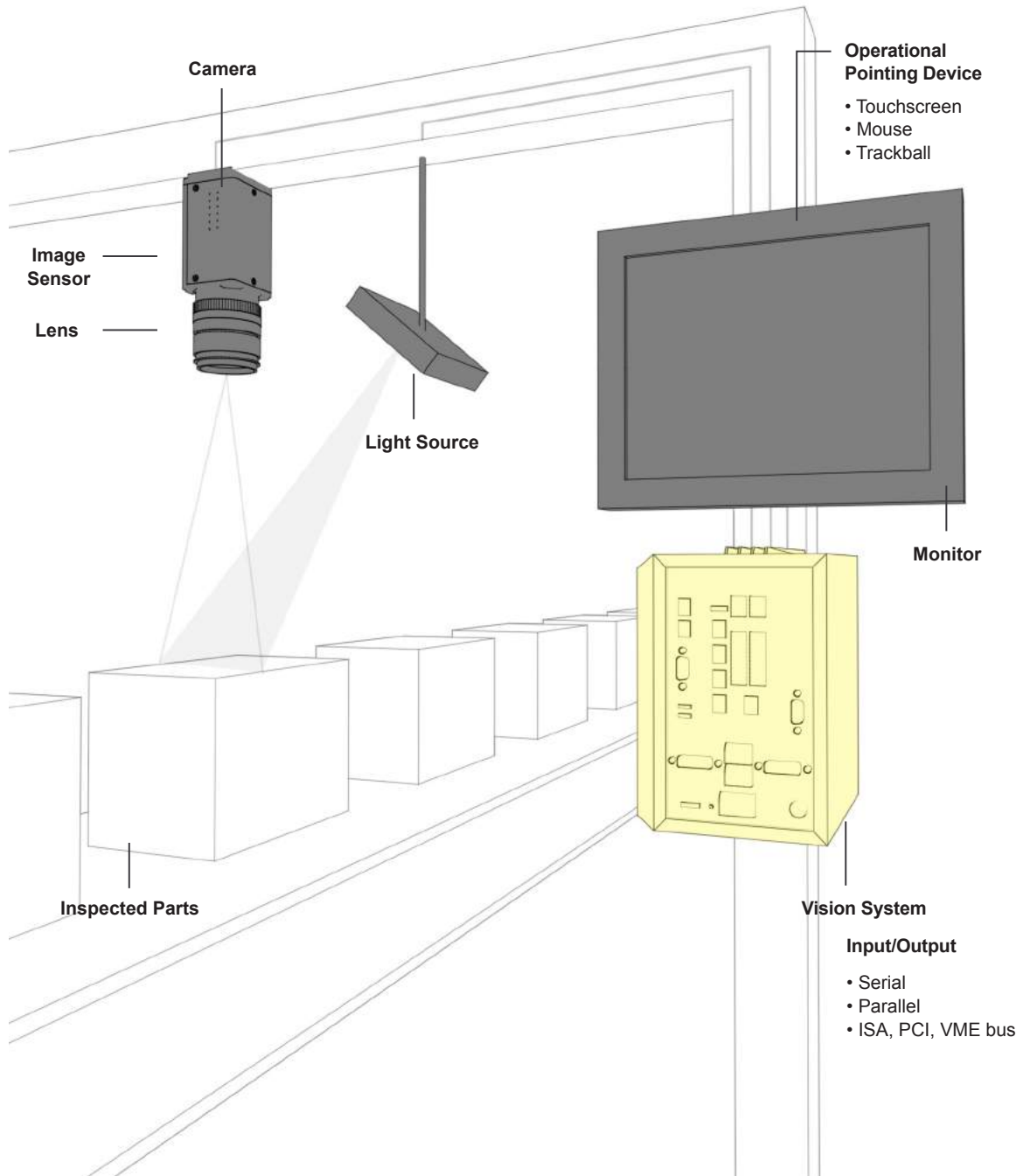
Figure 9. Main components of a machine vision system.
